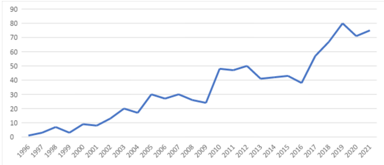
Figure 1: Citations to Bresnahan & Trajtenberg (1995) in Web of Science
